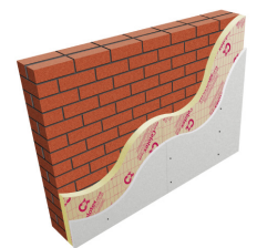
Direct fix
